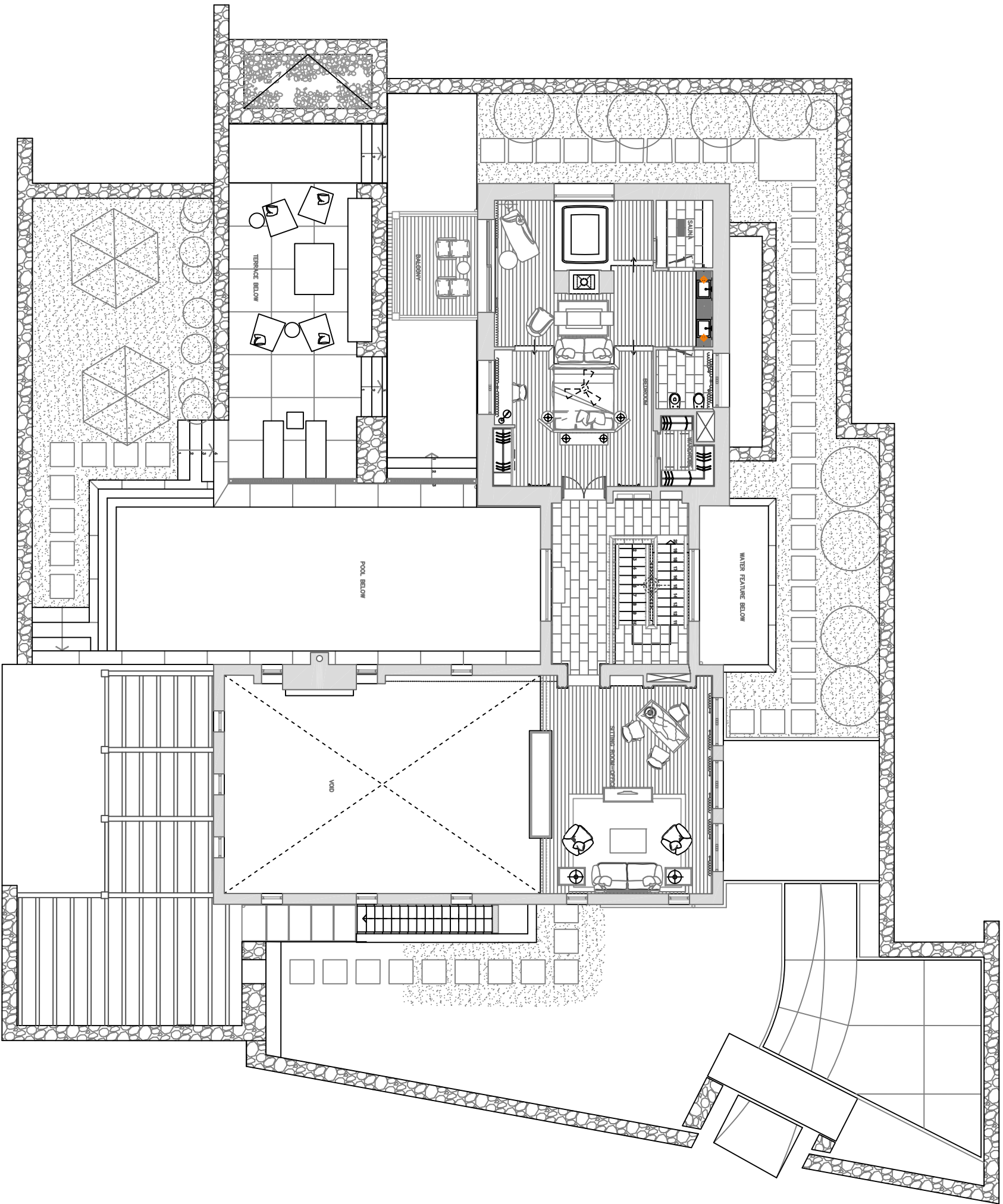
VILLA METHONI - FIRST FLOOR (SCALE 1:150 IN A3)
